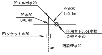
S6' 給水工詳細図 ±E2-3 0.3-20 L=0.5m L=0.5m×N=1
