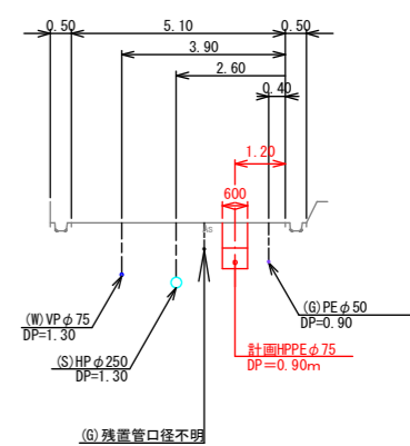
J-J'
